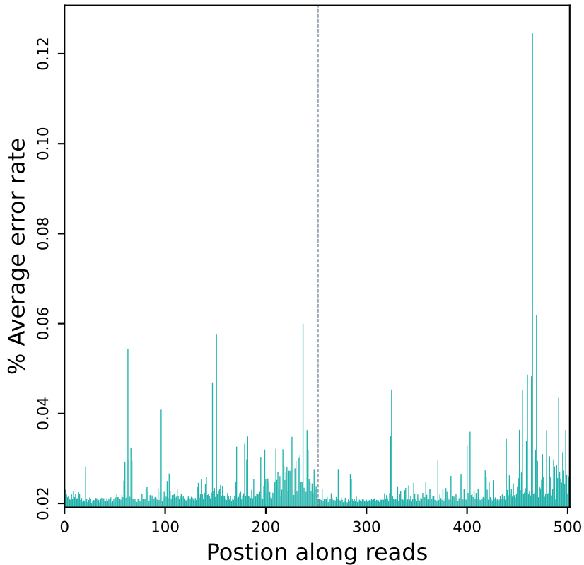
Error rate distribution along reads (R20113)
